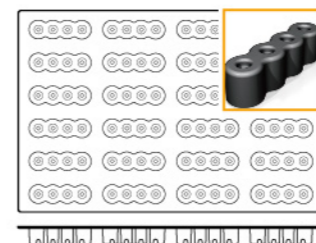
70.421.20.0098 28连转角模 590x390x50mm 中型52x52x50.7mm 容积约: 102ml
