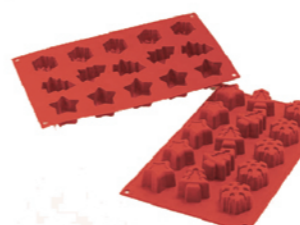
SF136 15连圣诞节模 300x175x25 单个39x49 h25 体积约: Tot337.5ml
